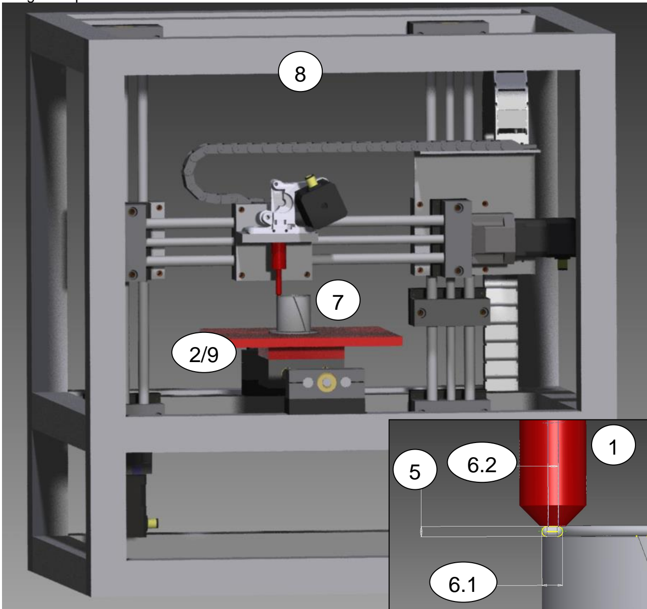
Image: 3D-printer
